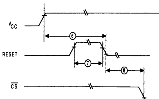
Timing Diagram 2. RESET Timing
