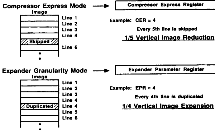
Figure 17. CEP Express and Granularity Modes
