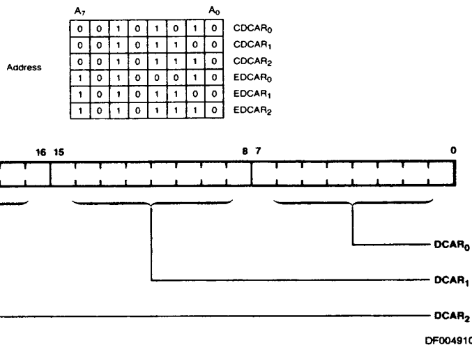
Figure 43. Destination Current Address Registers (CDCAR, EDCAR)
