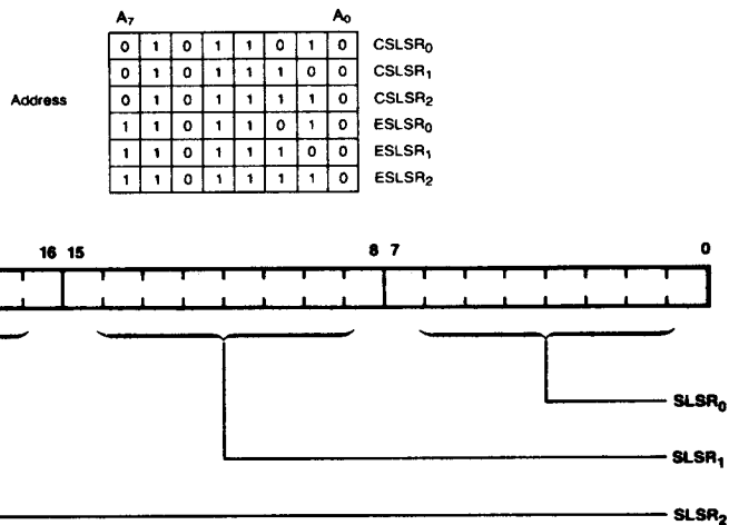
Figure 39. Source Line Start Address Registers (CSLSR, ESLSR)
