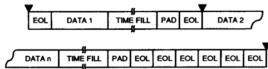
Figure 63. Byte Boundary Conditioned with Auto EOL and Time Fill
