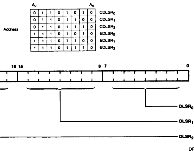
Figure 44. Destination Line Start Address Registers (CDLSR, EDLSR)
