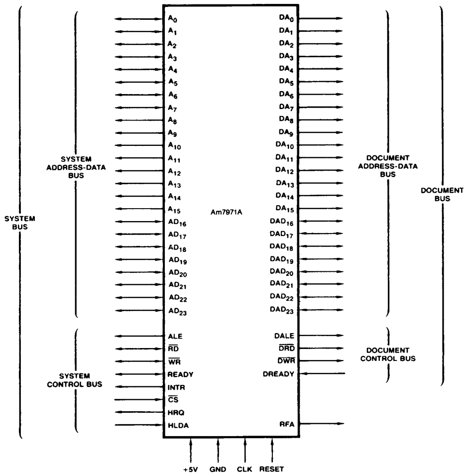
Figure 5. Am7971A Logic Symbol
