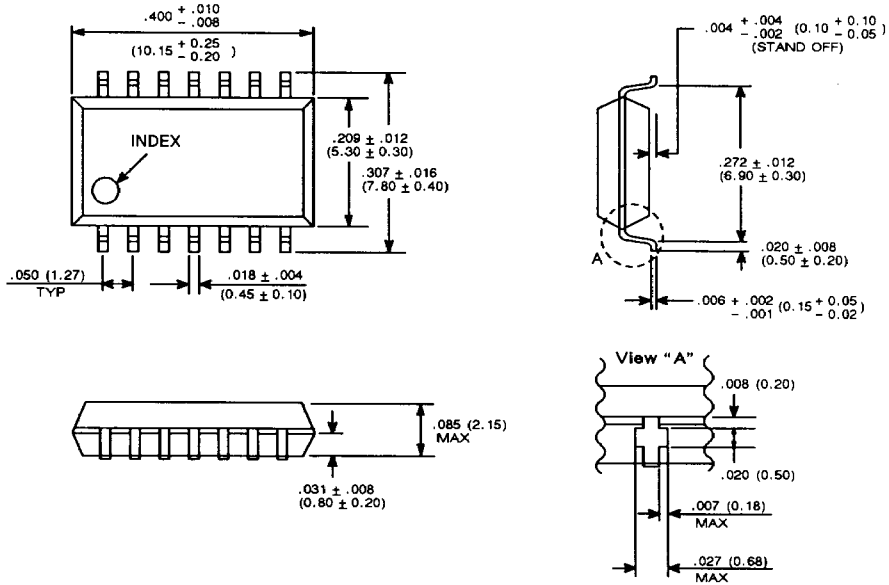
14-LEAD PLASTIC FLAT PACKAGE (CASE No.: FPT-14P-M01)
