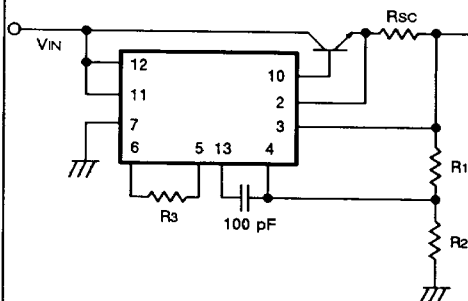
Fig. 14 - POSITIVE VOLTAGE REGULATOR NPN TRANSISTOR
