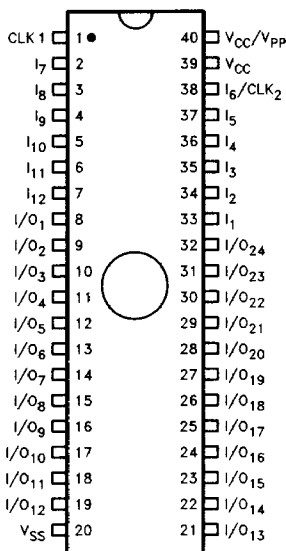
Pin Configuration
